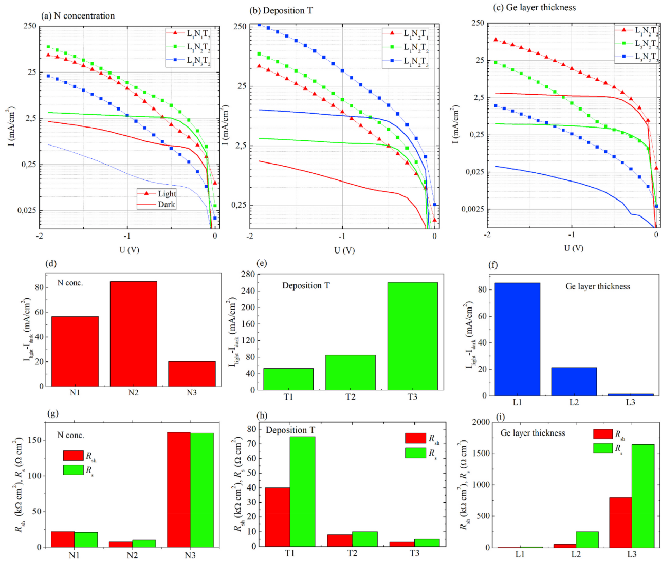
Fig. 8. (a)–(c) I–V curves of the annealed films for a bias voltage between 0 and 2 V, (d)–(f) difference between current generated in dark and light at a bias voltage of 1.8 V for three series of the films. (g)–(i) Shunt and serial resistances ( R_{\text{sh}} and R_{\text{s}} respectively), determined from the dark current measurements.
