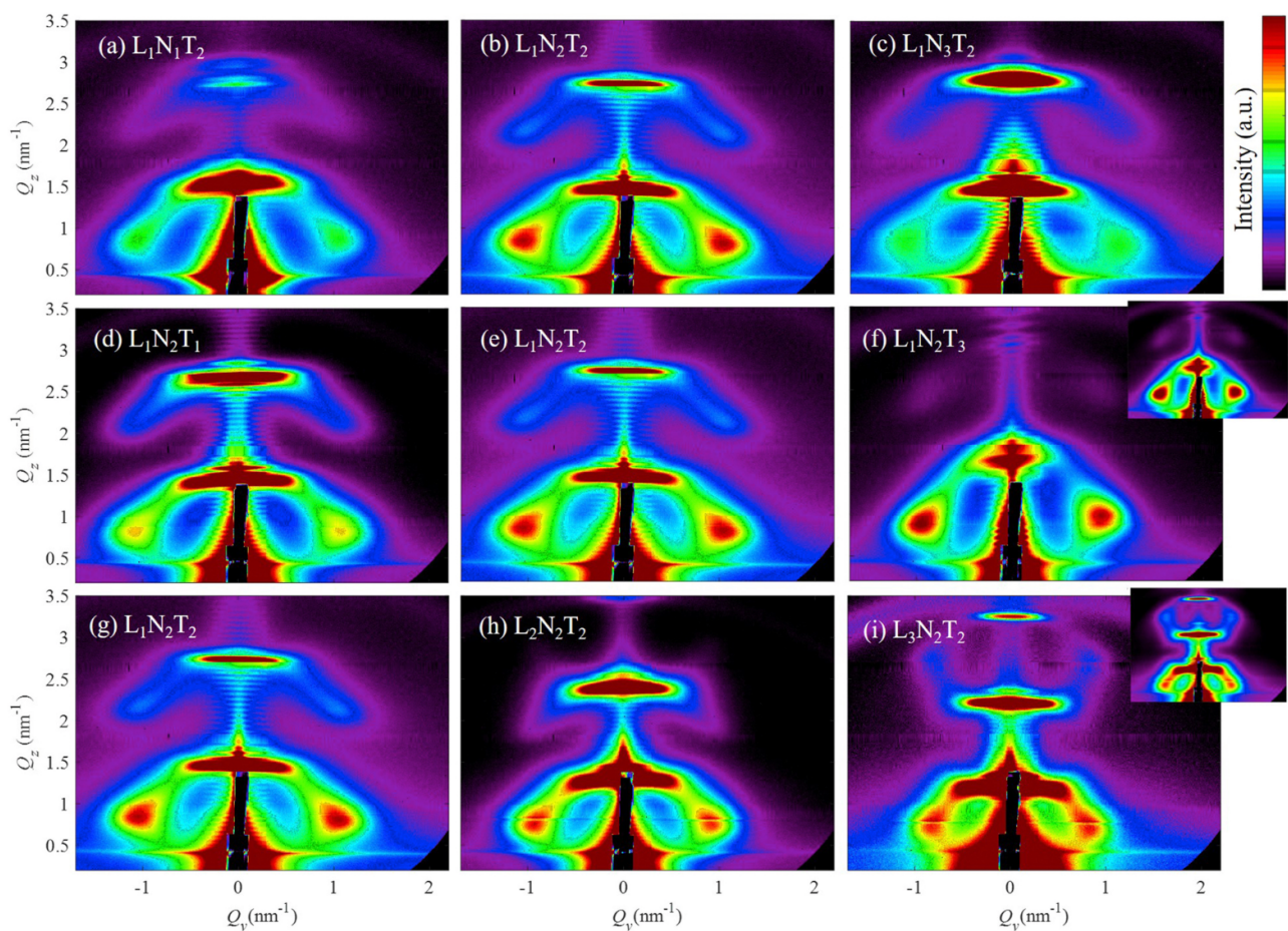
Fig. 1. GISAXS maps of the films. (a)–(c) nitrogen content is increasing, (d)–(f) deposition temperature is increasing and (g)–(i) Ge layer thickness is increasing. The GISAXS maps of the annealed films are practically the same as the non-annealed. Two examples are shown in the insets of the panels (f) and (i).
