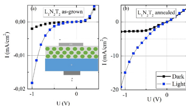
Fig. 7. I–V curves of the (a) as-grown and (b) annealed film L_1N_2T_2 . The scheme of the geometry for the measurement is shown in the inset of panel (a).
