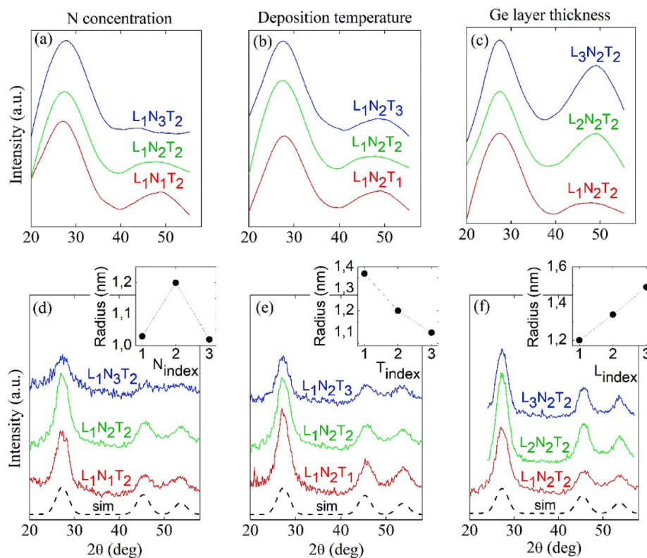
Fig. 4. XRD spectra of all samples after (a)–(c) deposition and (d)–(f) annealing in vacuum for 45 min. The simulated curves of crystalline Ge QDs are shown by dashed lines. The insets show the c-Ge QD radii obtained from the fitting of the corresponding diffraction curves. The X-axis in the insets indicates the number of the changing index in the sample name for each series.
